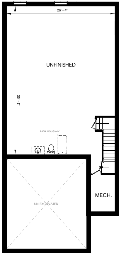
BASEMENT - 1,084 SQ. FT.
