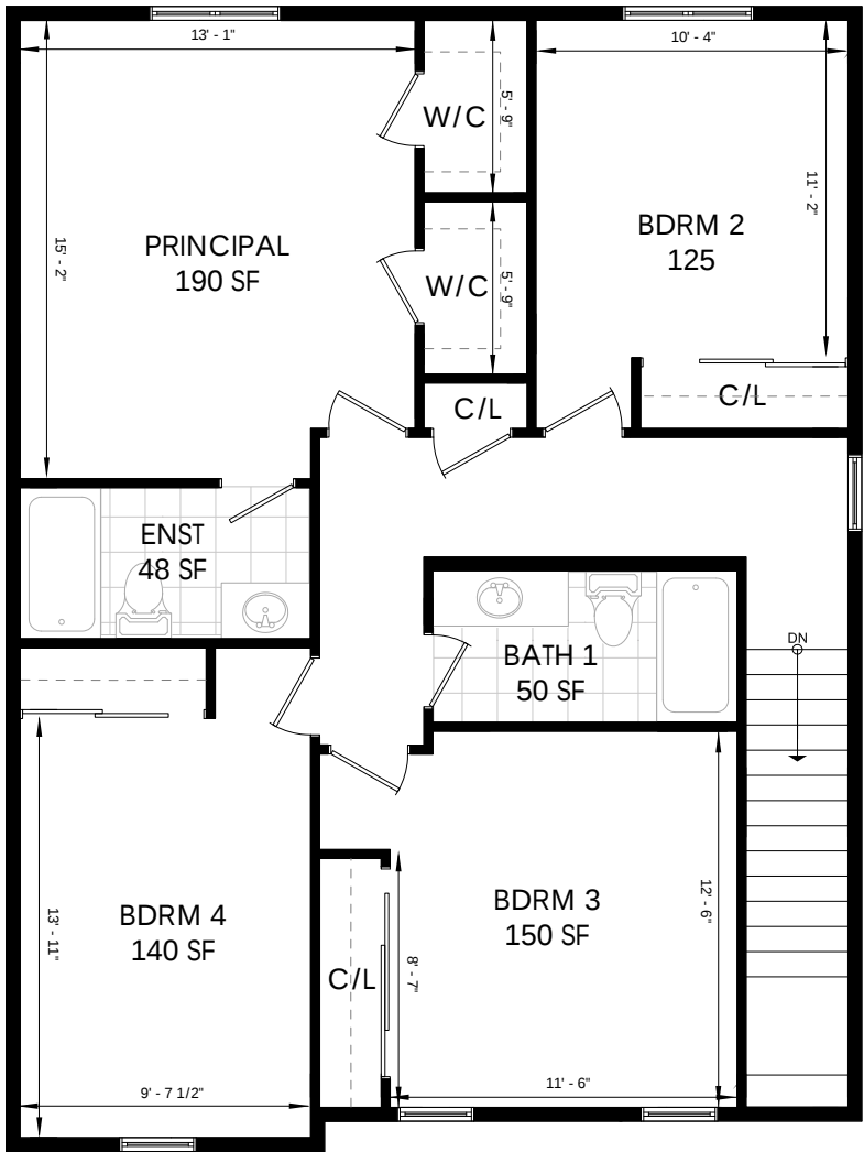
SECOND LEVEL 1040 SQ. FT.
