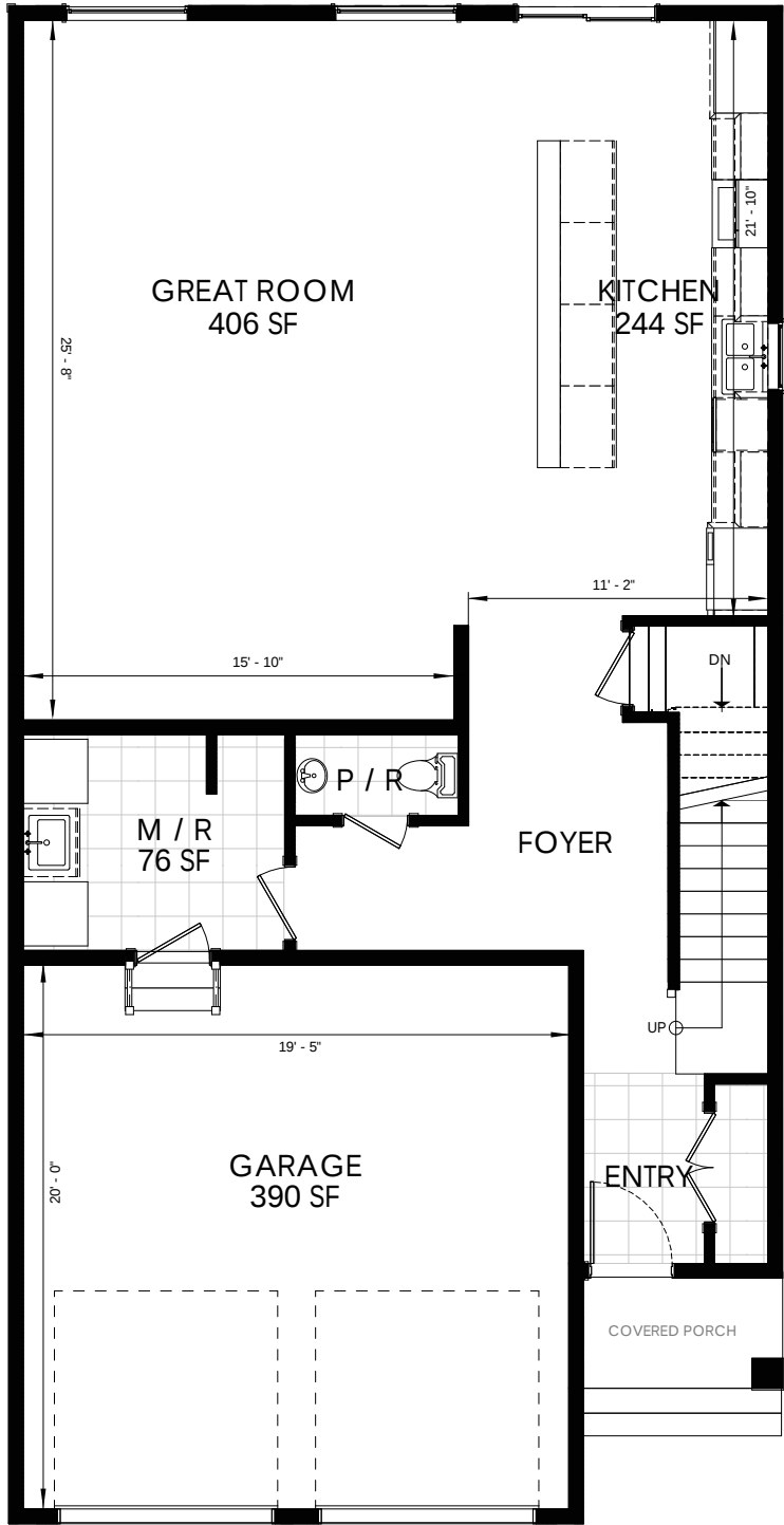
MAIN LEVEL - 1,085 SQ. FT.
