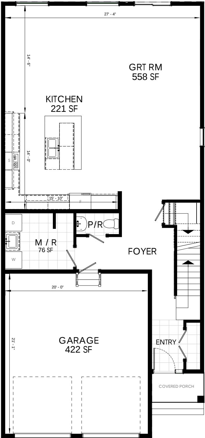
MAIN LEVEL - 1,316 SQ. FT.
