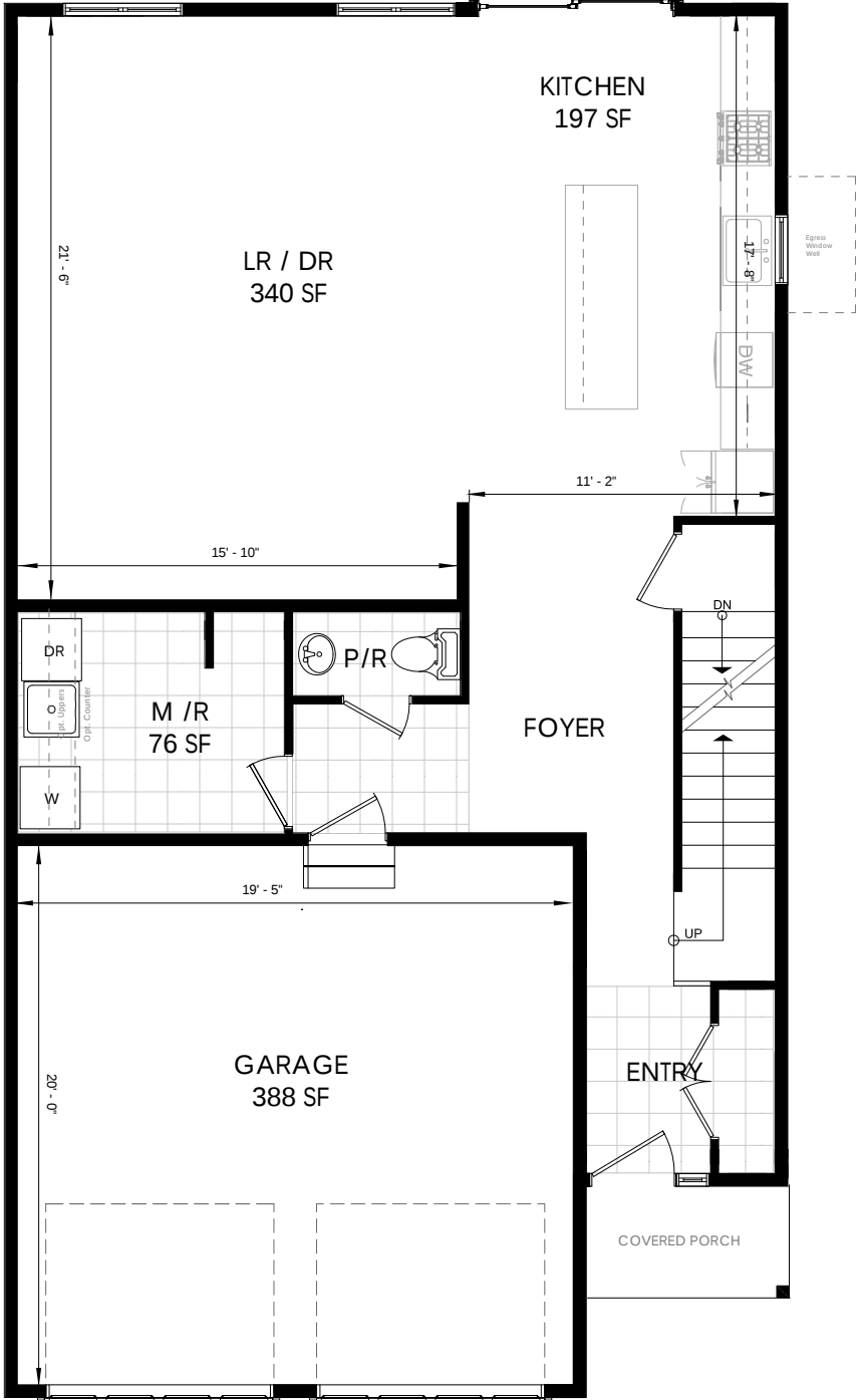
MAIN LEVEL 960 SQ. FT.
