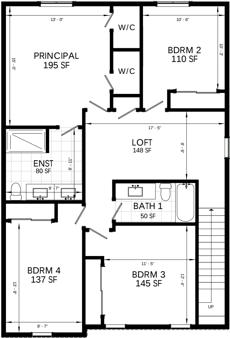
SECOND LEVEL - 973 SQ. FT.
