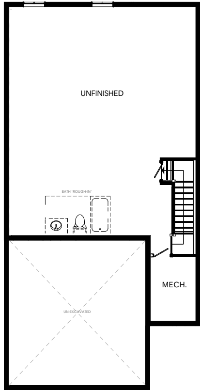
BASEMENT - 973 SQ. FT.
